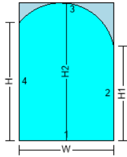
076SH - ARCH-STRAIGHT SIDES OFFSET RIGHT...
