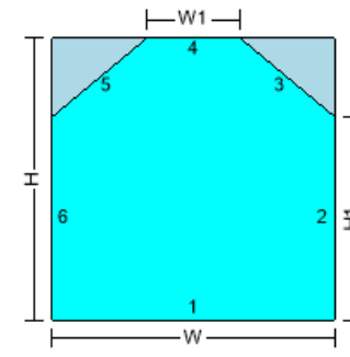
238SH - HEXAGON-STRAIGHT SIDES
