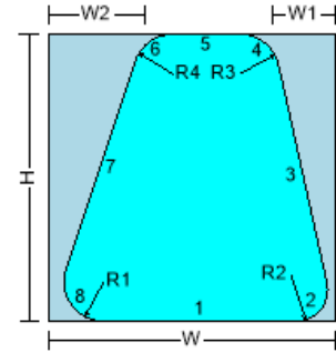
113SH - TRAPEZIUM-4 RADIUS CORNERS
