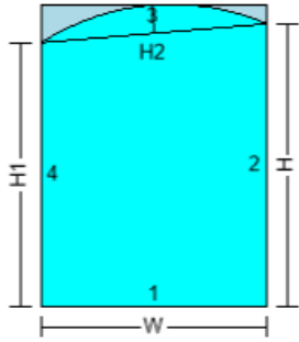
069SH - ARCH-STRAIGHT SIDES OFFSET LEFT (R...
