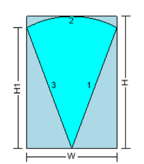
401SH - CONE (LEG HEIGHT)
