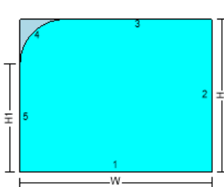
255SH - RECTANGLE-1 RADIUS CORNER LH (LEG...
