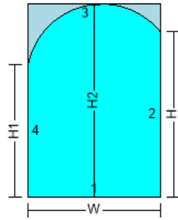
077SH - ARCH-STRAIGHT SIDES OFFSET LEFT (F...
