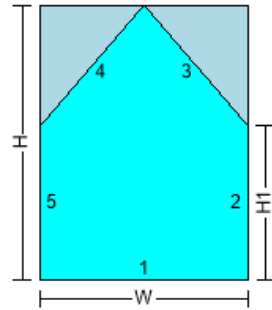
215SH - PENTAGON-STRAIGHT SIDES
