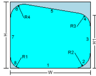
103SH - RAKE RH-4 RADIUS CORNERS
