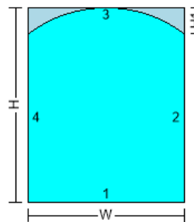
065SH - ARCH-STRAIGHT SIDES (RISE)
