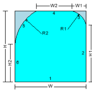
156SH - RECTANGLE-2 RADIUS CORNER (RADIUS)
