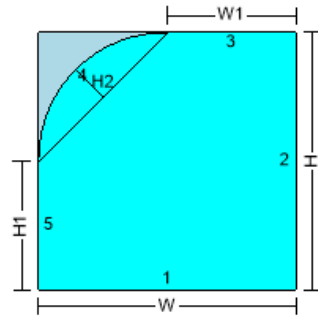
155SH - RECTANGLE-1 RADIUS CORNER LH (RISE)
