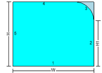
254SH - RECTANGLE-1 RADIUS CORNER RH (LE...
