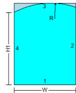
067SH - ARCH-STRAIGHT SIDES OFFSET LEFT (R...
