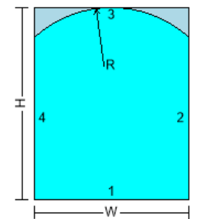
064SH - ARCH-STRAIGHT SIDES (RADIUS)
