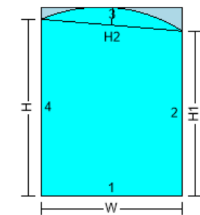
068SH - ARCH-STRAIGHT SIDES OFFSET RIGHT...
