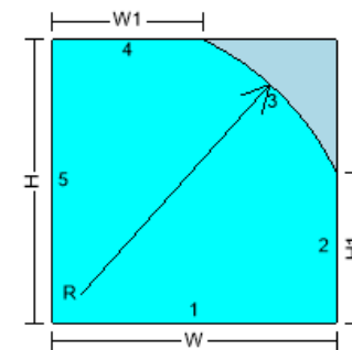
152SH - RECTANGLE-1 RADIUS CORNER RH (RA...
