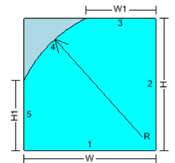
153SH - RECTANGLE-1 RADIUS CORNER LH (RA...
