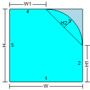
154SH - RECTANGLE-1 RADIUS CORNER RH (RIS...
